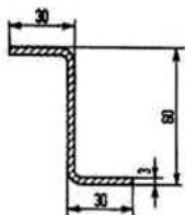
Z 30/60/30 x 3
