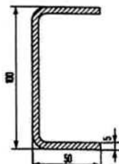
U 50/100/80 x 5
