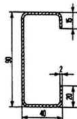
C 20/40/90/40/15 x 2
