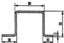
Omega 30/50/60/50/20 x 3
